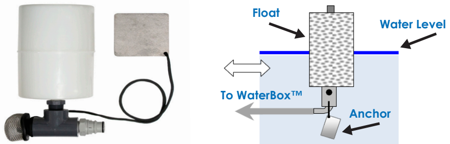
Figure 4: Schematic of the use of the float intake device
