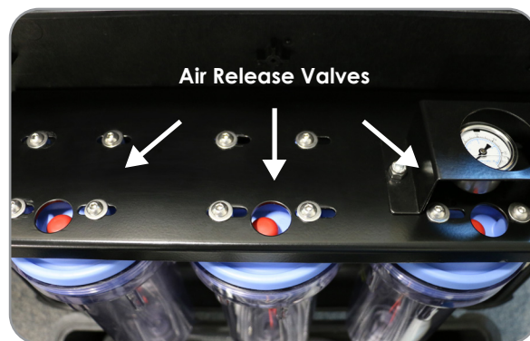
Figure 7: Air release valves on filter housing
