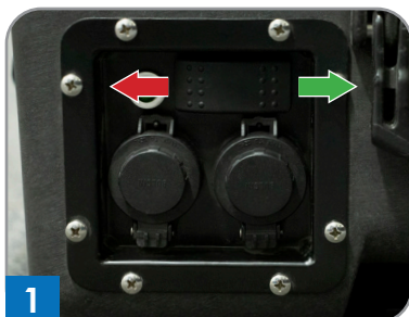
1 Switch To Left For DC Power Switch To Right For AC Power Switch To Center For Off
